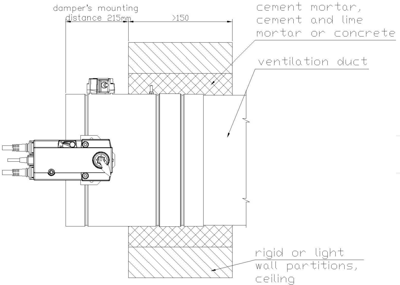
Figure 11. Installation method of fire dampers KTS in high wall thickness constructions
