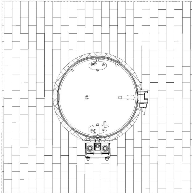
Figure 4. Installation of KTS in rigid wall construction with vertical axis of rotation of the damper.
