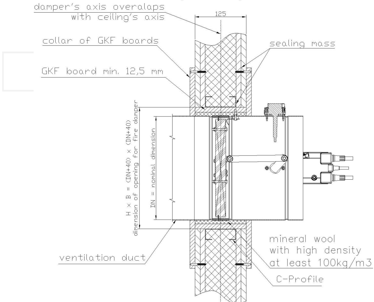
Figure 10. Installation method of fire dampers KTS in flexible wall with 125 [mm] thickness
