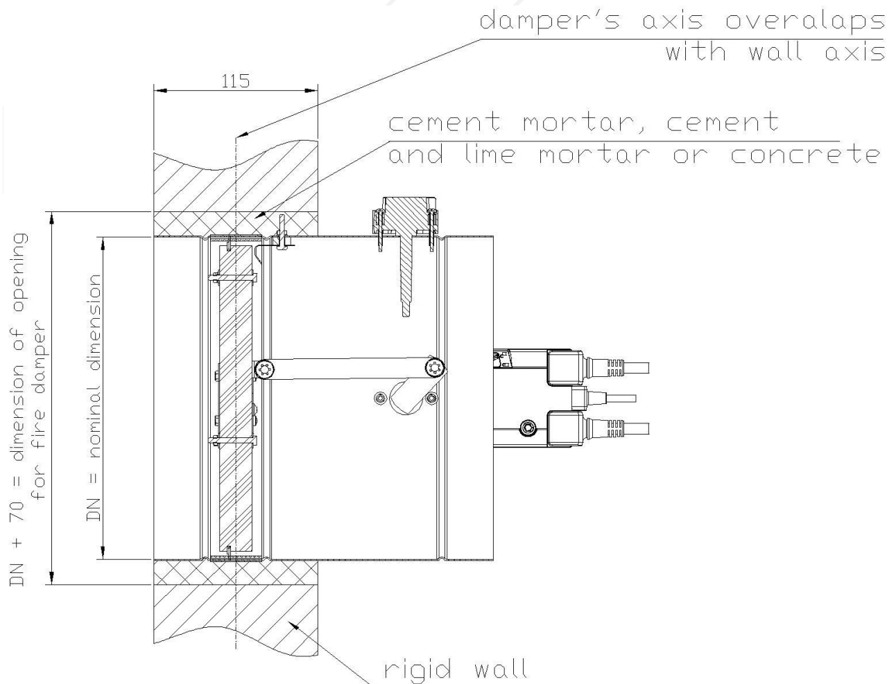
Figure 5. Installation of KTS in rigid wall construction with 115 [mm] wall thickness.
