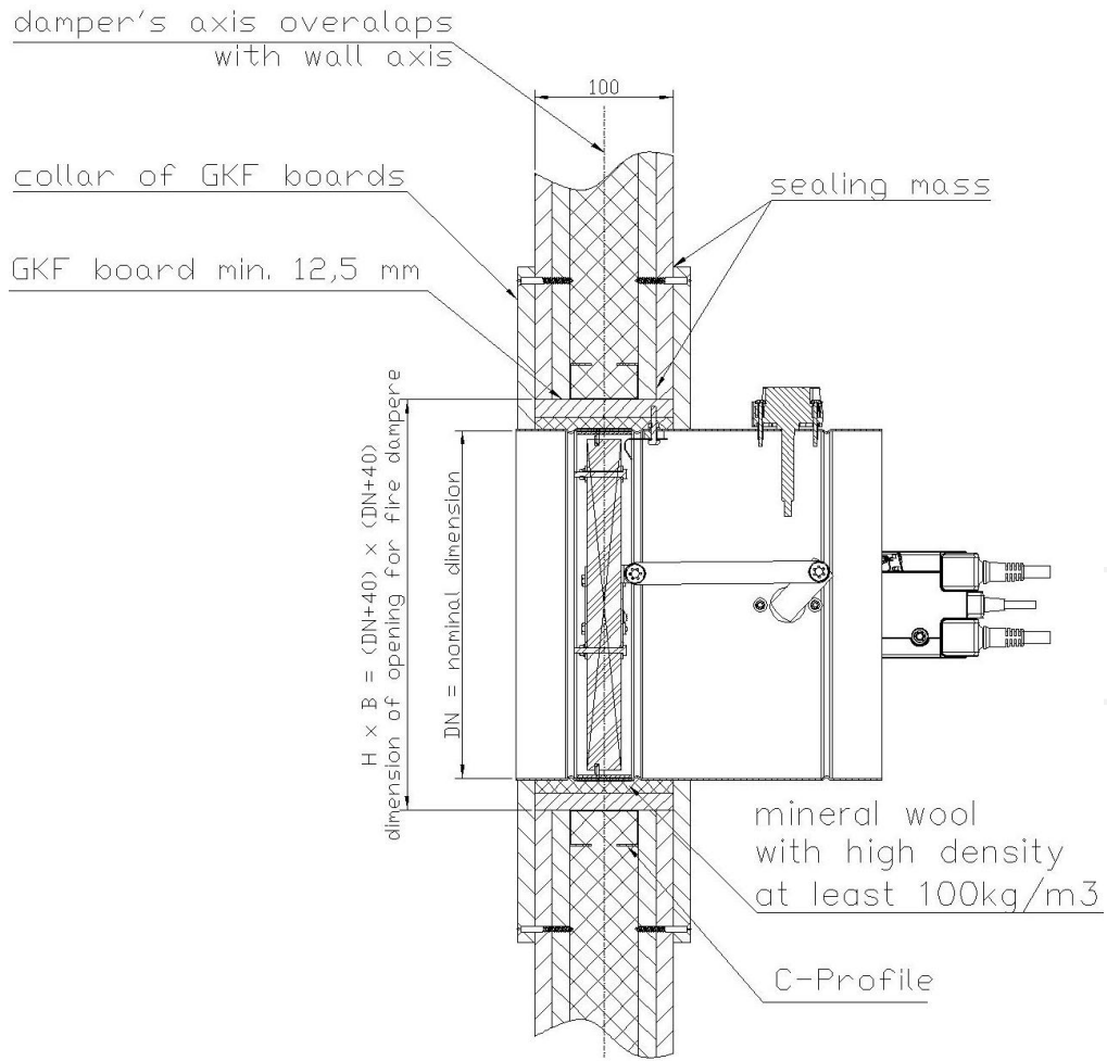
Figure 7. Installation method of fire dampers KTS in flexible wall with 100 mm thickness
