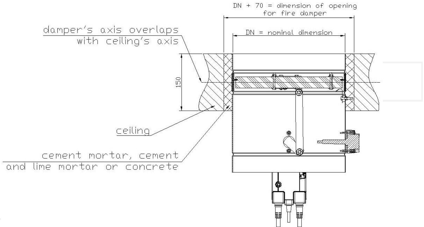
Figure 1. Installation method of fire dampers KTS in ceiling
