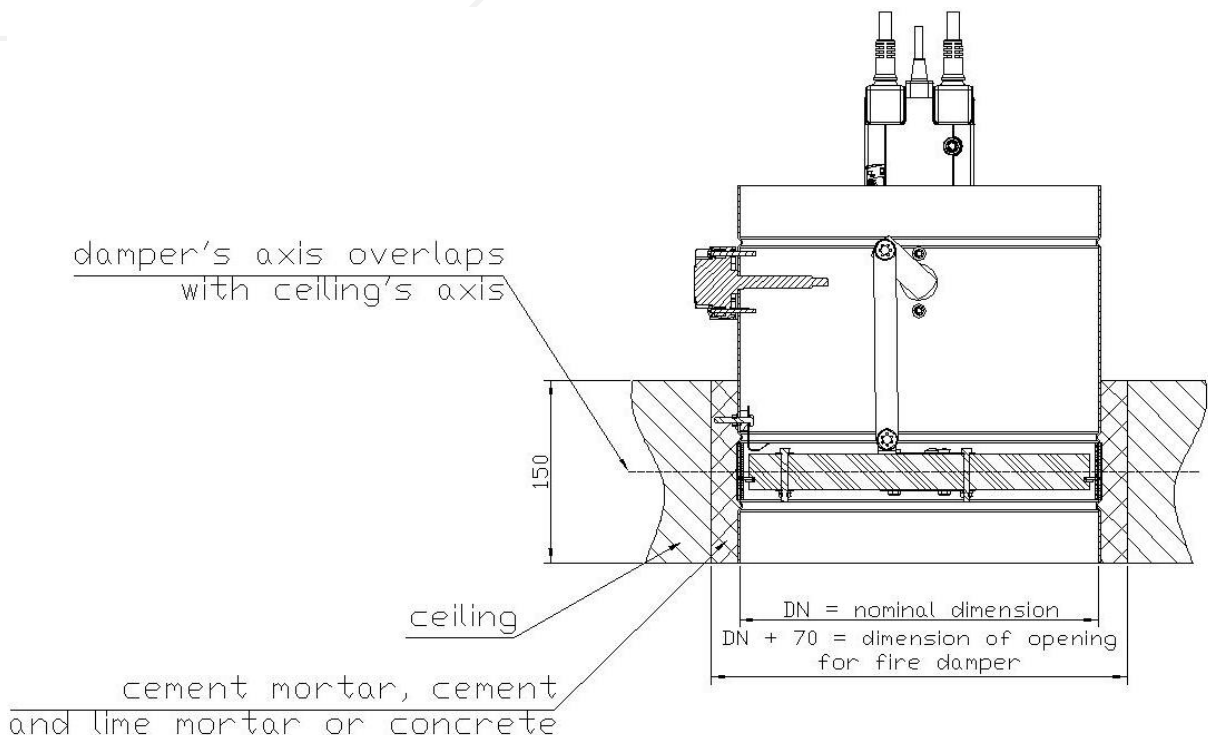
Figure 2. Installation method of fire dampers KTS in ceiling
