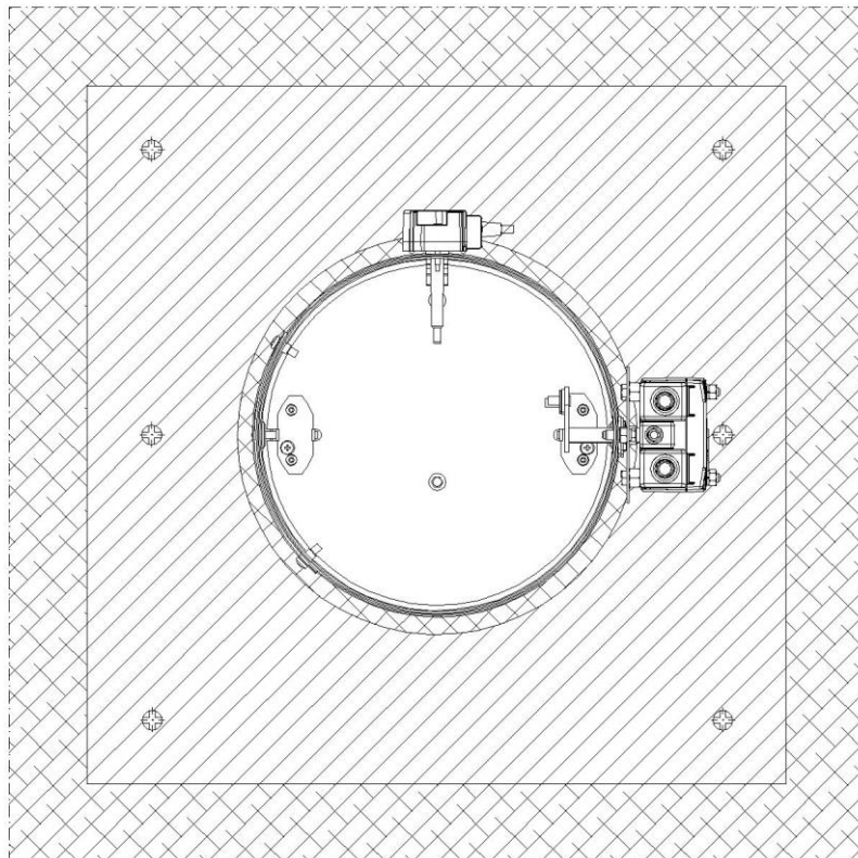
Figure 8. Installation method of fire dampers KTS in flexible wall with horizontal rotation axis of baffle
