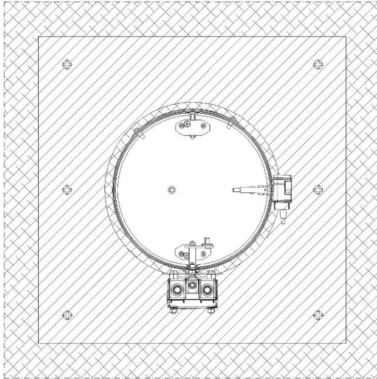
Figure 9. Installation method of fire dampers KTS in flexible wall with vertical rotation axis of baffle
