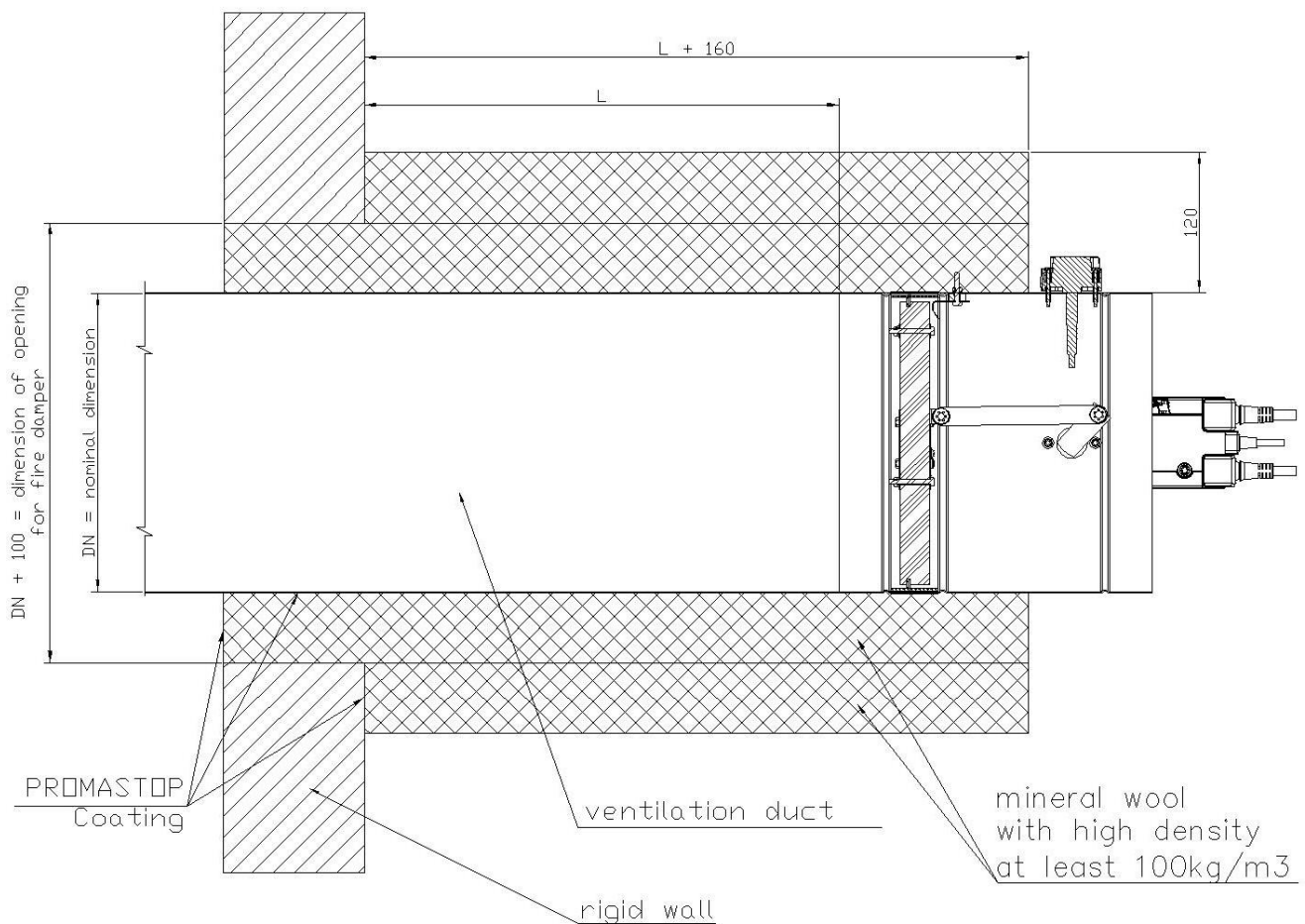
Figure 12. Installation method of fire dampers KTS away from wall constructions
