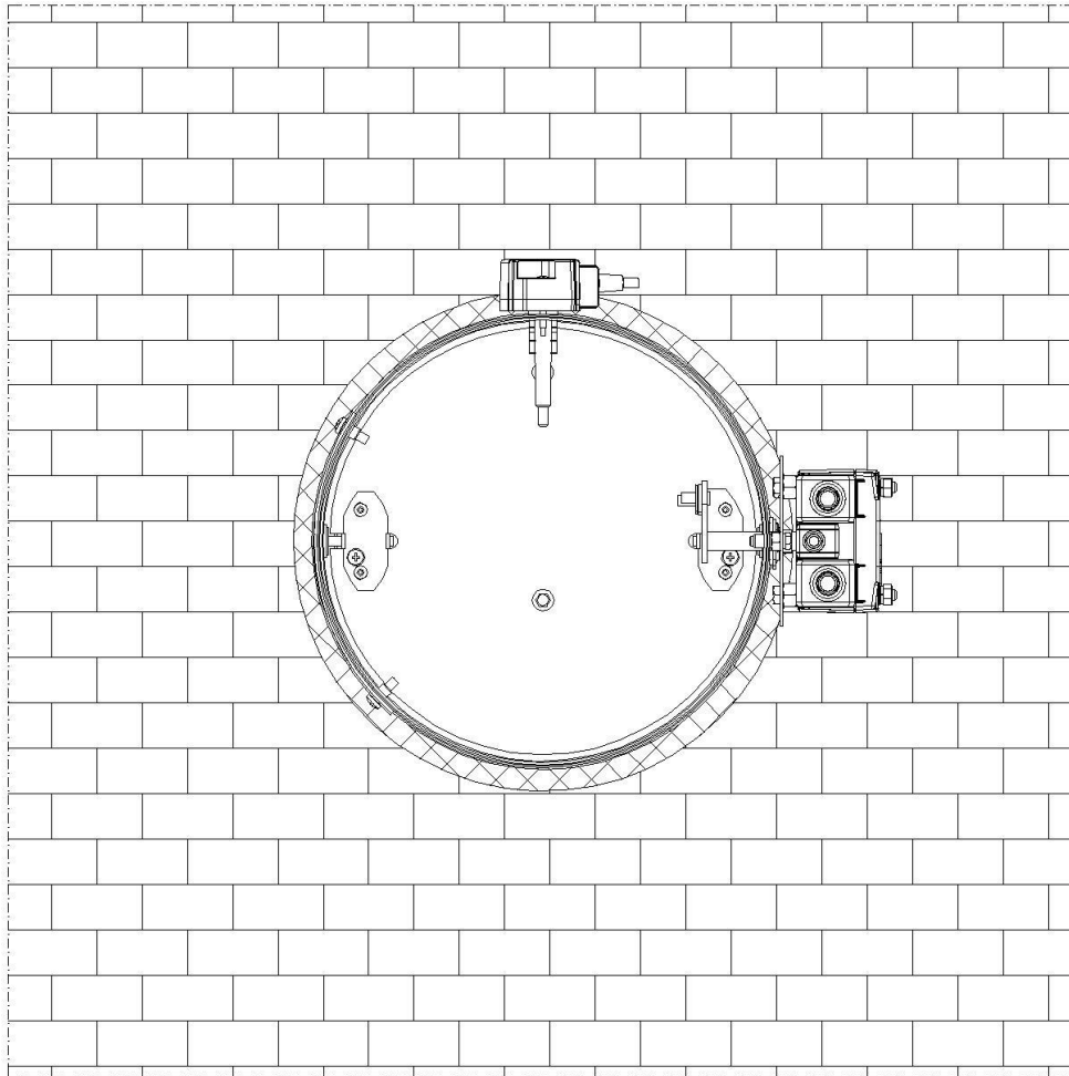
Figure 3. Installation of KTS in rigid wall construction with horizontal axis of rotation of the damper.
