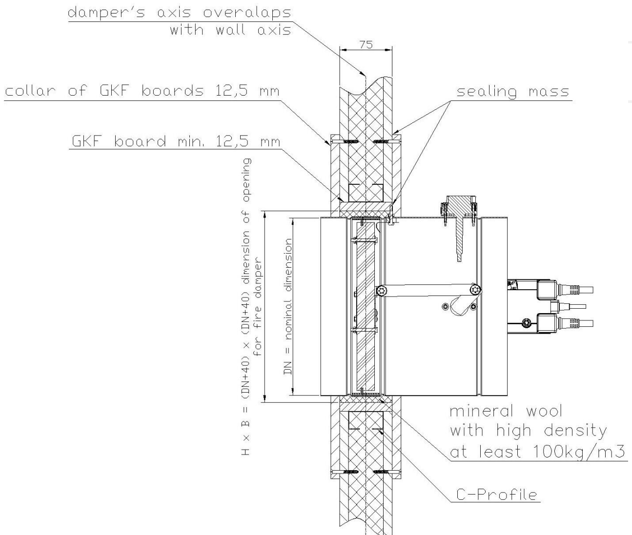
Figure 6. Installation of KTS in flexible wall construction with 75 [mm] thickness
