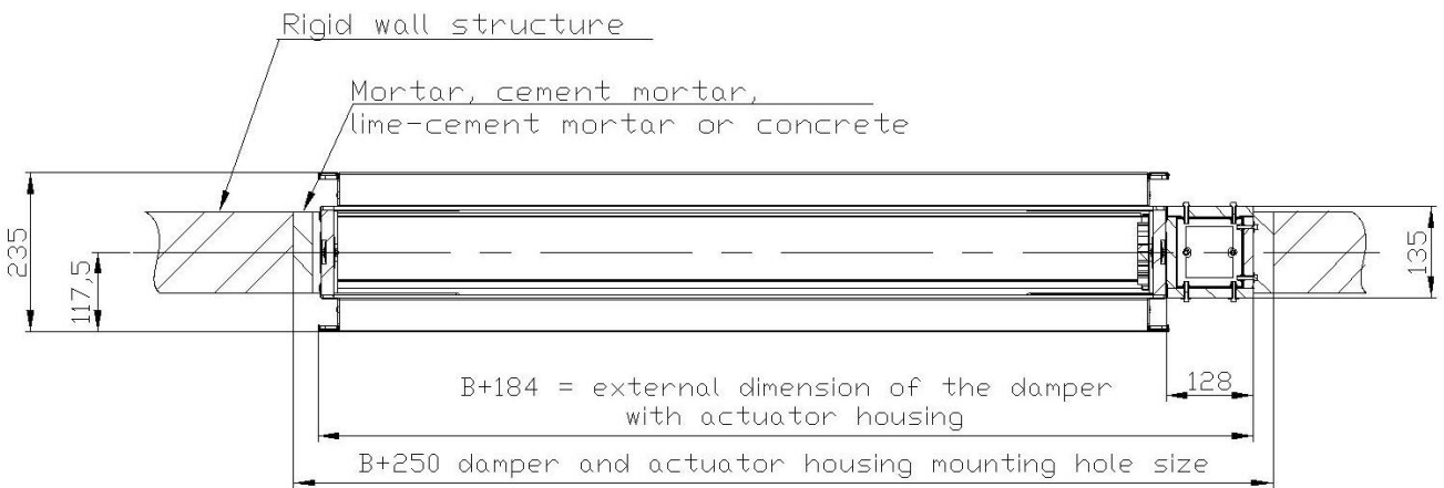
Figure 3. Installing method of WKP-O fire dampers in rigid wall
