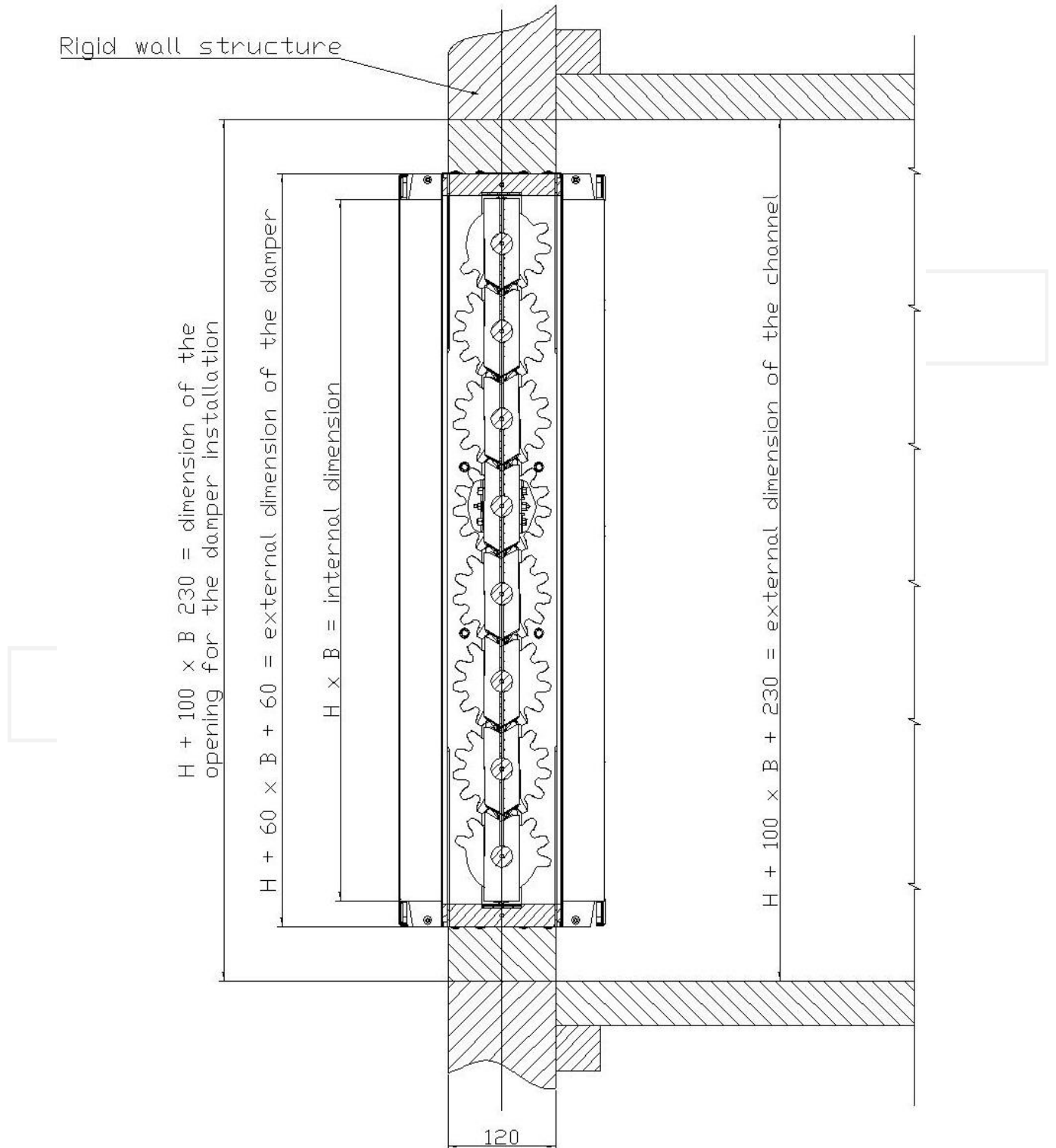
Figure 5. Installing method of WKP-O fire dampers with PROMAT boards duct.
