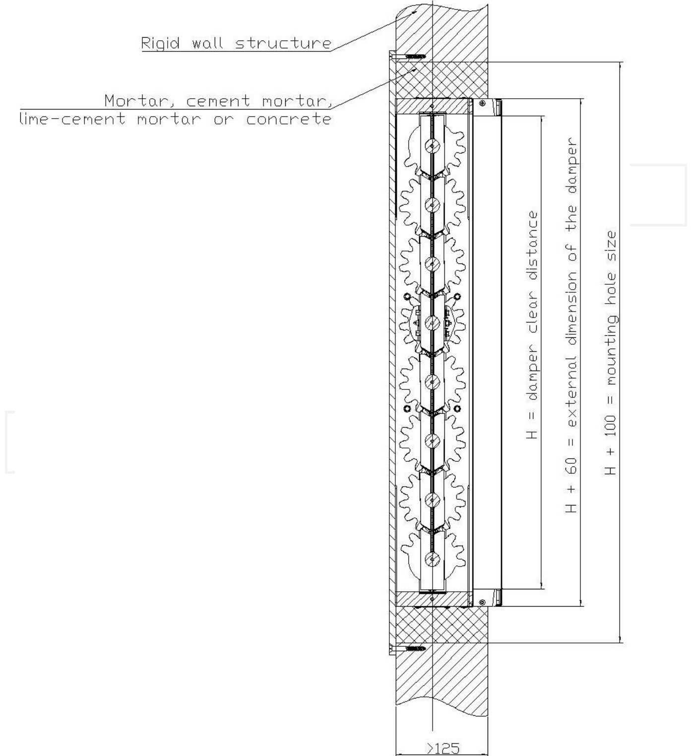
Figure 6. Installation method of fire dampers WKP-O in structures thicker than 125 mm
