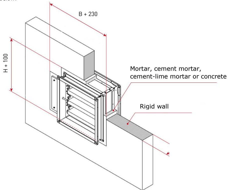
Figure 1. Dimensions of the installation opening of the WKP-O dampers in rigid wall with a horizontal and with vertical axis of rotation of the baffle, with planned cut for actuator housing. The C dimension is given in the table.
