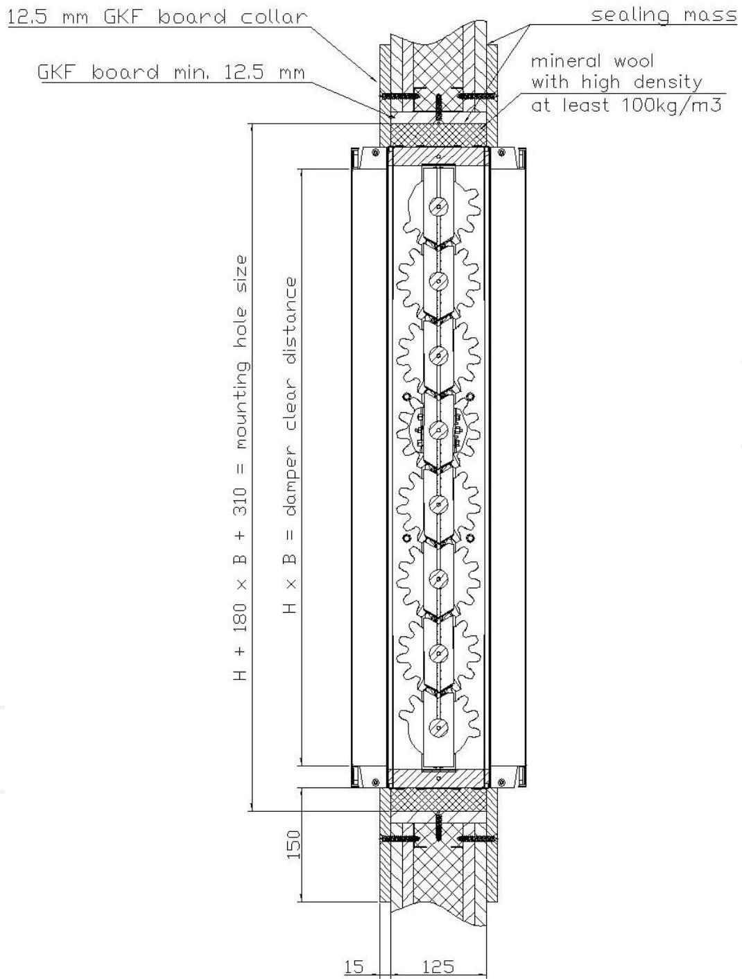
Figure 7. Installation method of fire dampers WKP-O in standard wall with 125 mm thick
