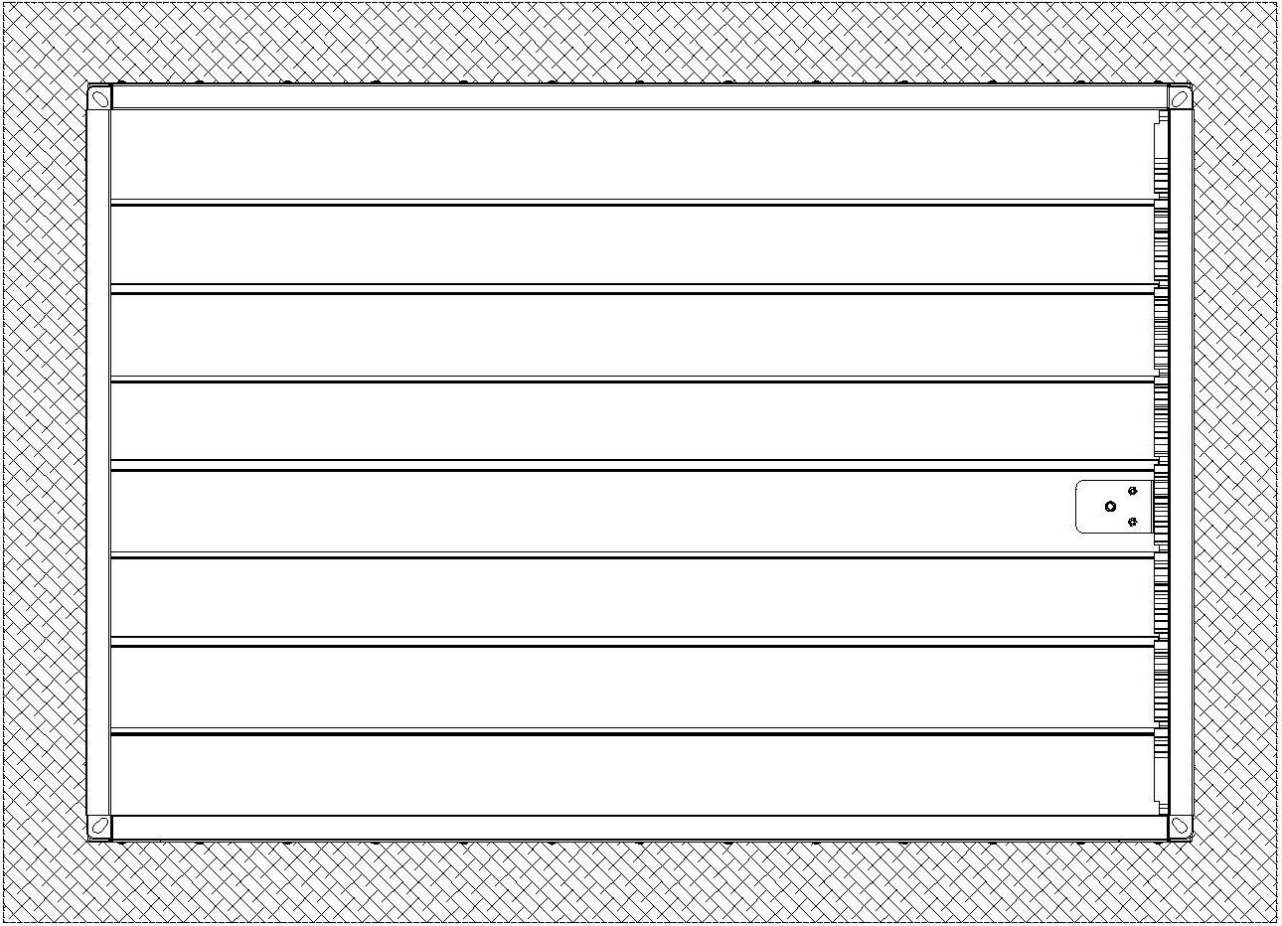
Figure 8. Installation method of fire dampers WKP-O in standard wall
