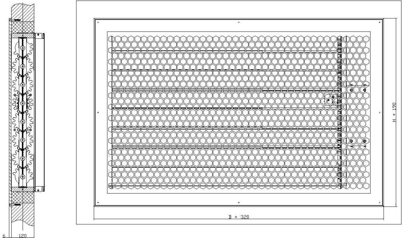
Figure 9. Installation method of MKW-B honeycomb mesh cover
