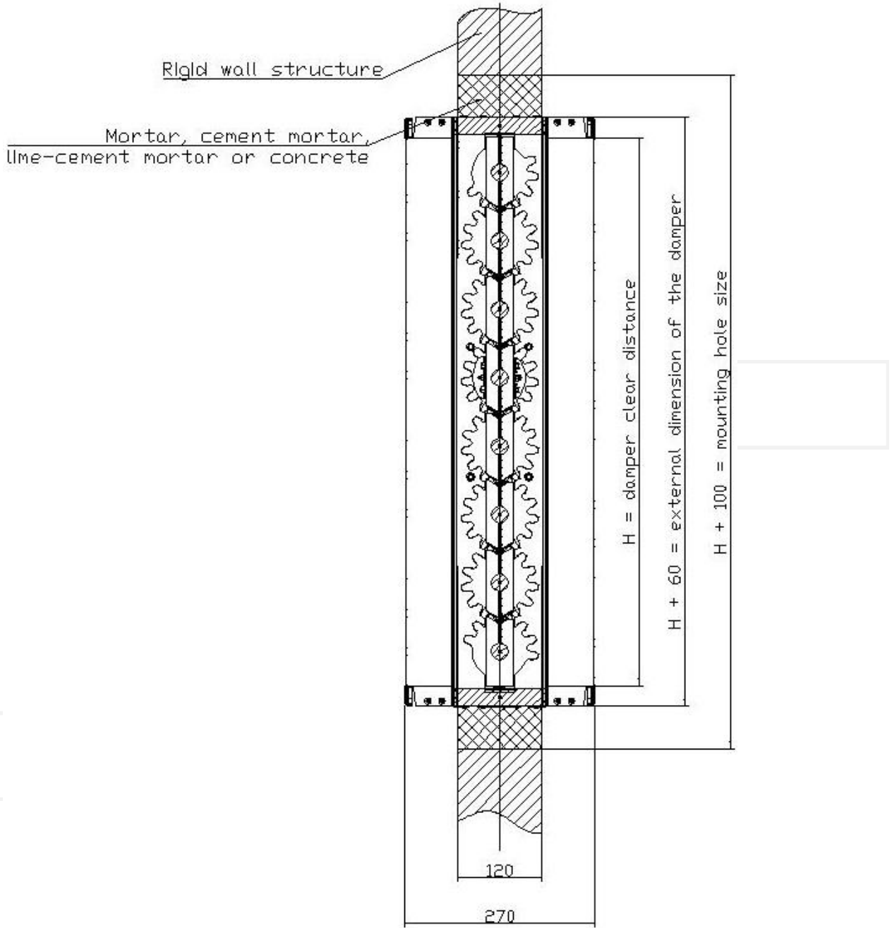
Figure 2. Installing method of WKP-O fire dampers in rigid wall.
