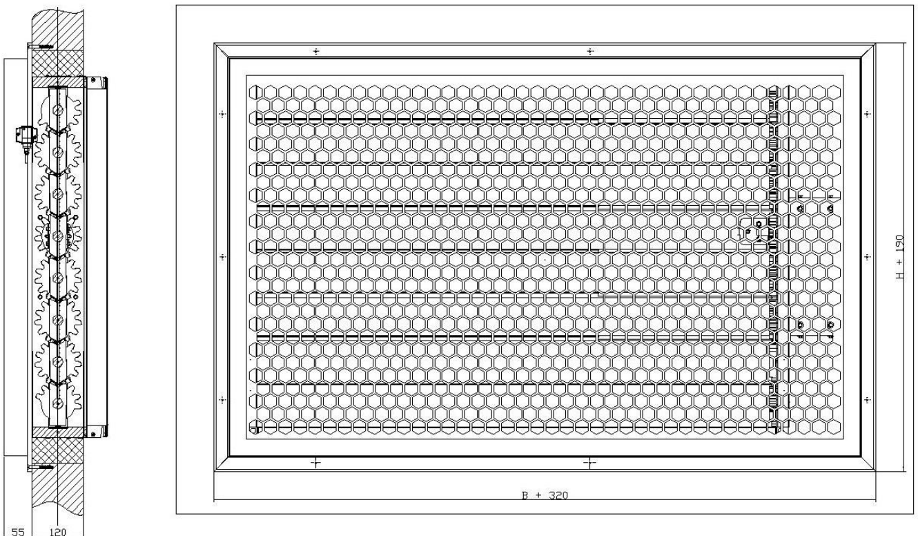
Figure 10. Installation method of MKW-D honeycomb mesh cover
