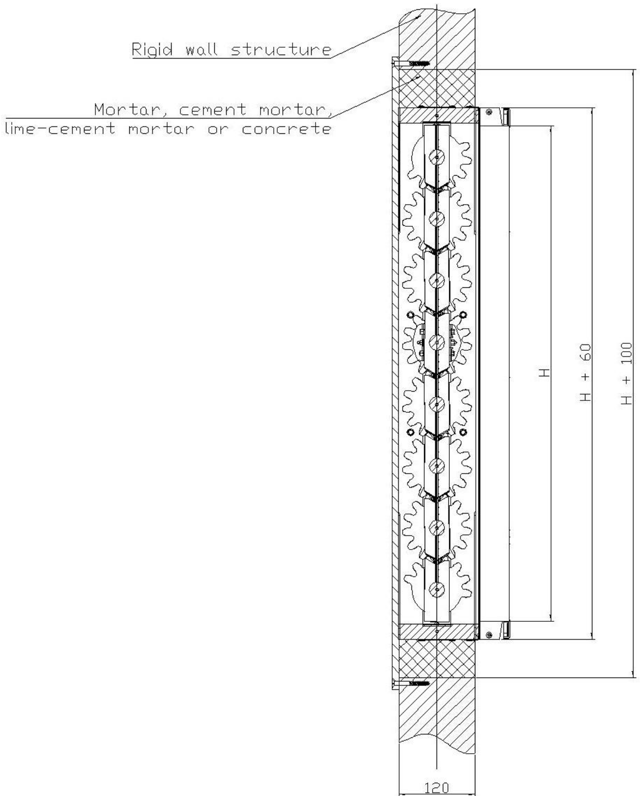
Figure 4. Installing method of WKP-O fire dampers in rigid wall with KST grille in rigid wall structure.
